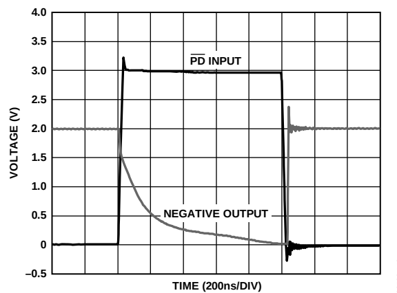
Figure 41. Power-Down Response Time
