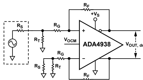
Figure 60. ADA4938-1/ADA4938-2 Configured for Unbalanced (Single-Ended) Input
